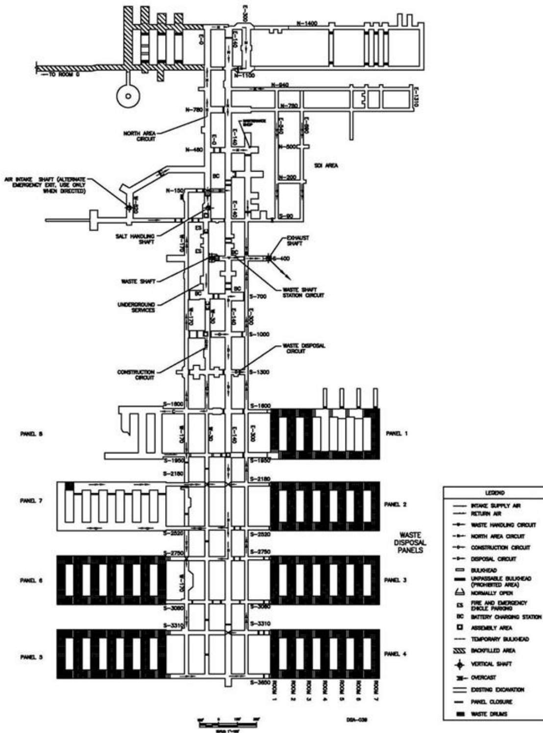
Figure 2.4-15. Underground Layout and Ventilation Flow
