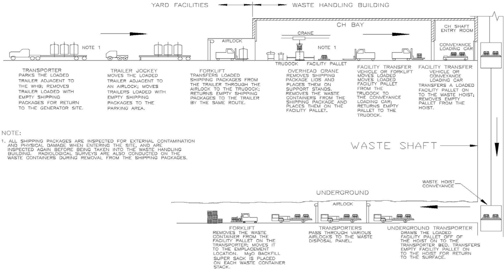
Figure 2.6-2. Contact-Handled Waste Handling Process
