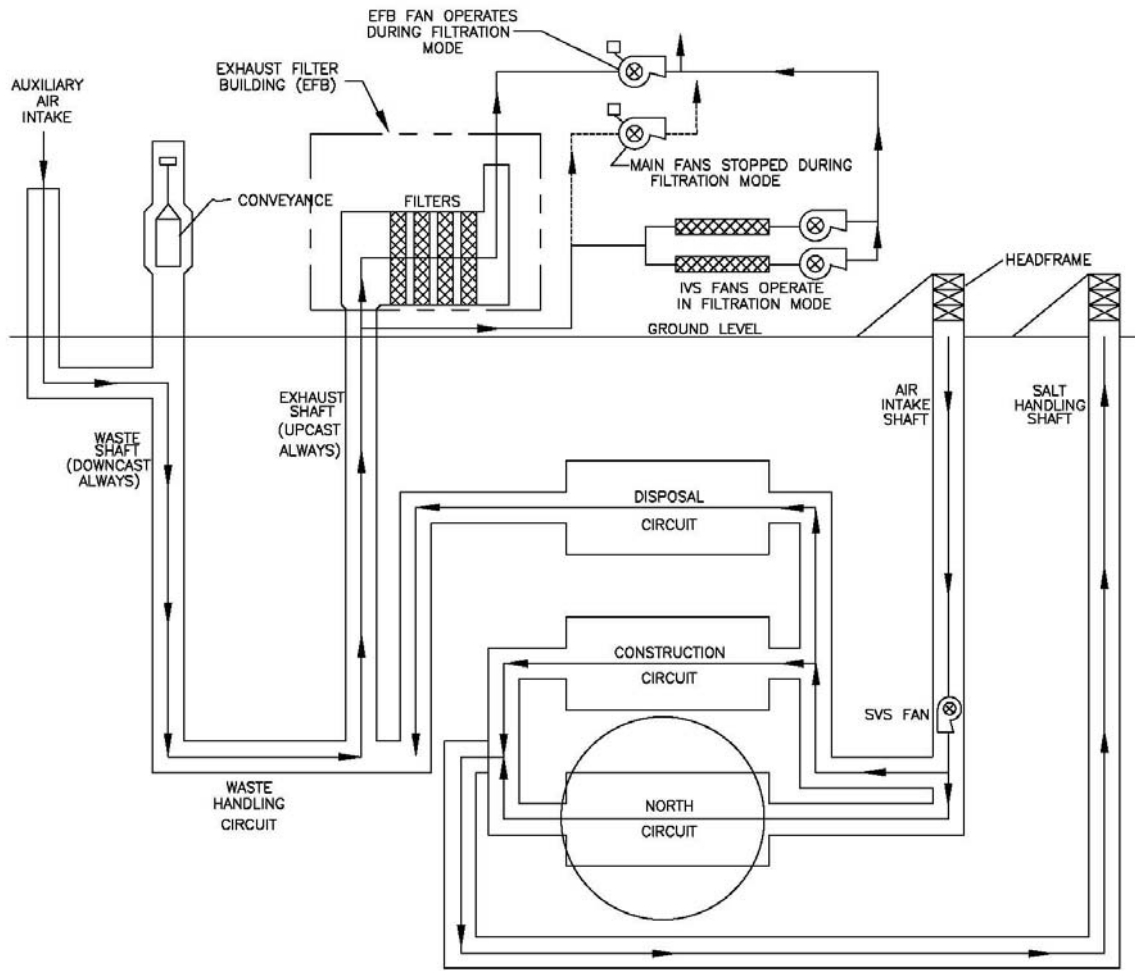
Figure 2.7-7. Underground Ventilation Airflow Diagram
