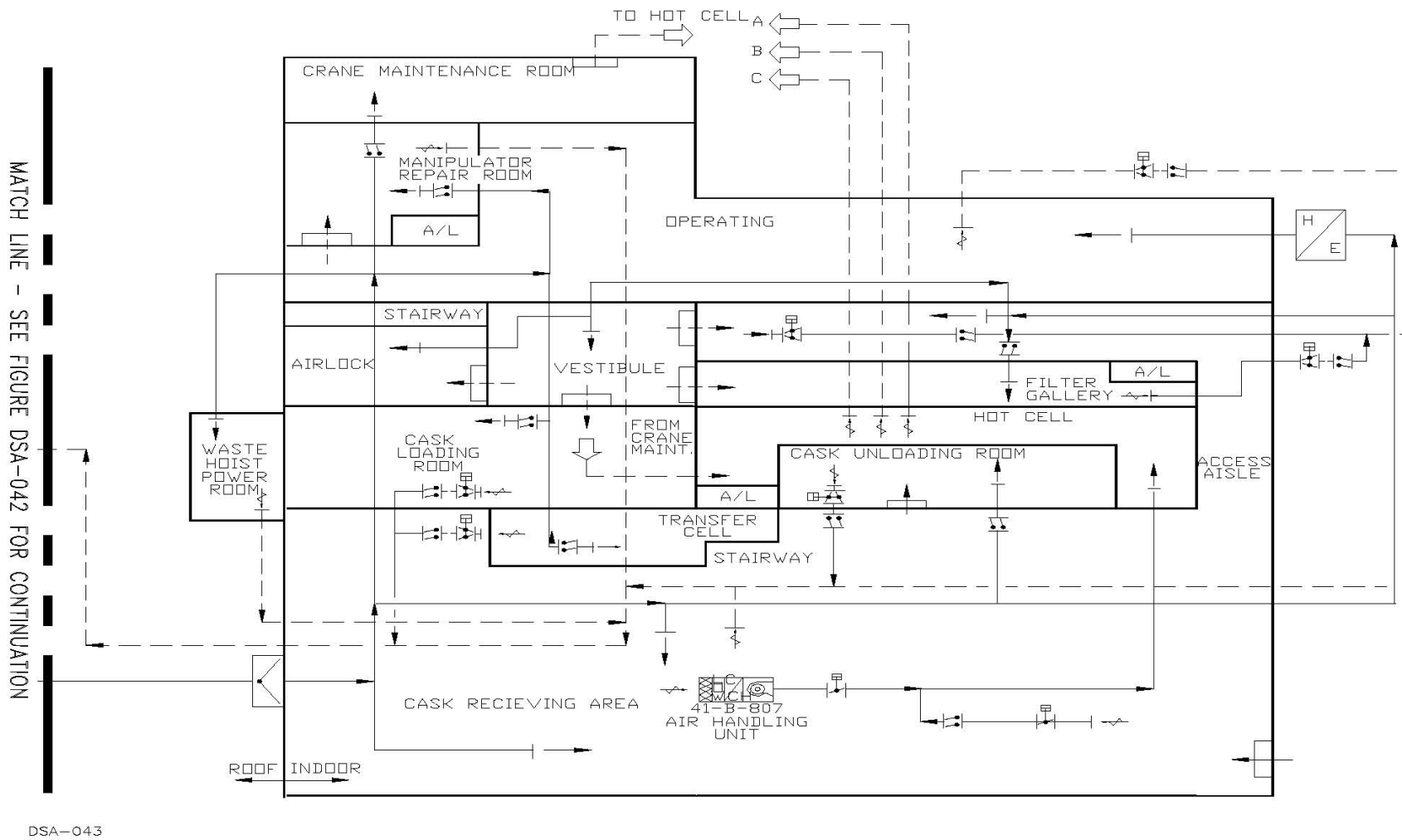
Figure 2.7-3. Waste Handling Building Remote-Handled HVAC Flow Diagram (continued)
