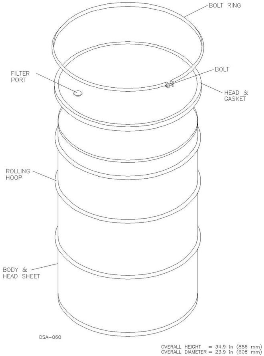
Figure 2.6-6. 55-gallon Drum
