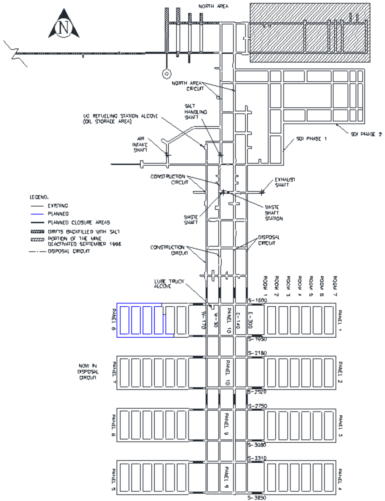
Figure 2.4-2. Underground Facilities
