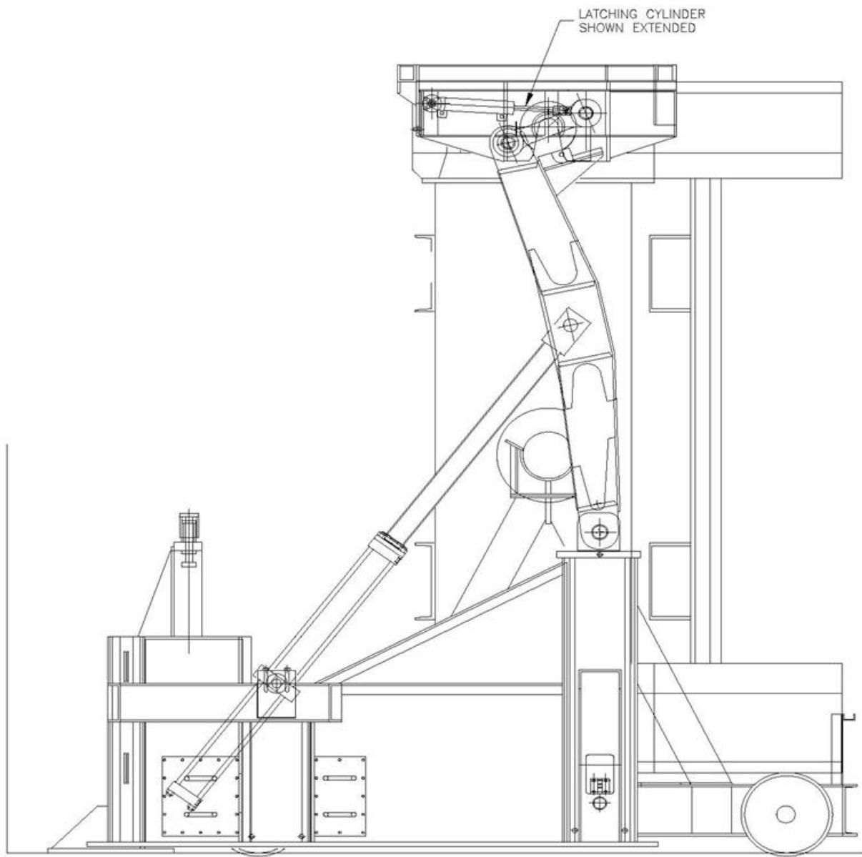
FRONT ELEVATION CASK VERTICAL
