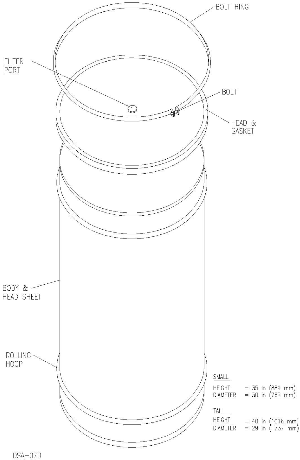
Figure 2.6-7. 85-gallon Drum
