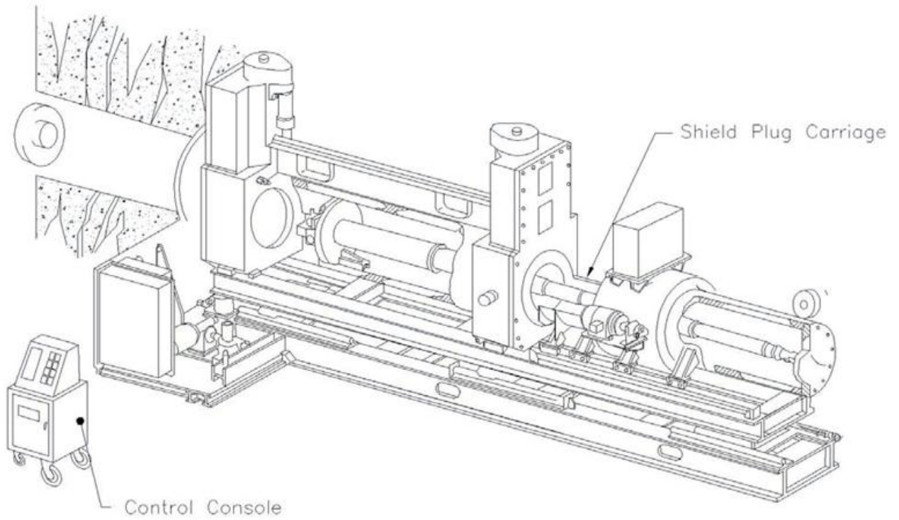
FACILITY CASK AGAINST SHIELD COLLAR. TRANSFER CARRIAGE RETRACTED. SHIELD PLUG CARRIAGE ON STAGING PLATFORM. SHIELD PLUG BEING INSTALLED.
